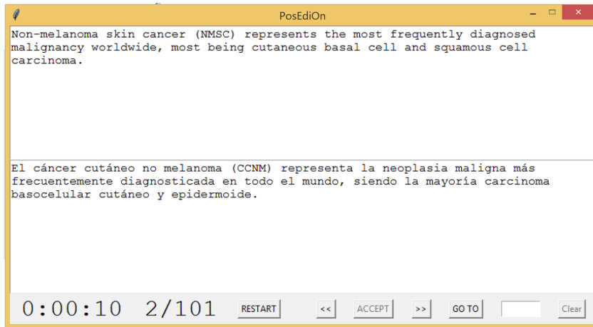
Figure 2: PosEdiOn interface
