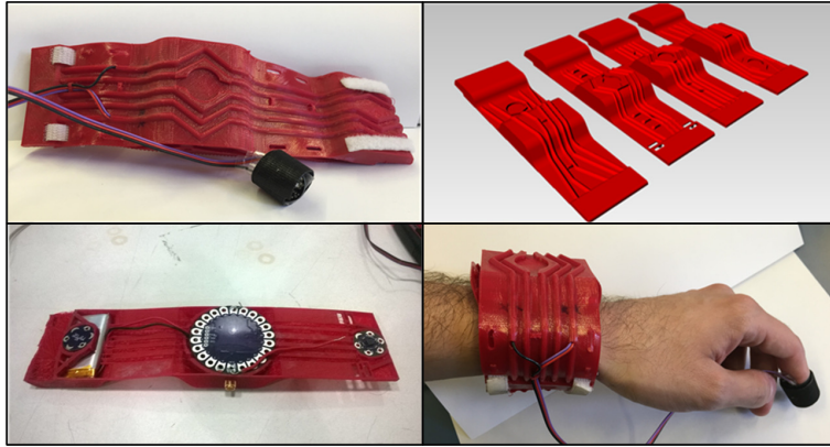
Figure 2: CUIDATS Wristband
