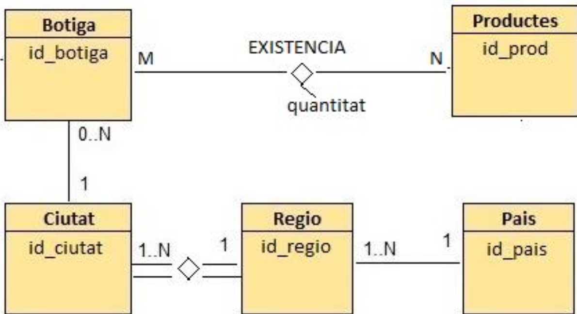
Figura 9: Diagrama conceptual E/R del ERP
