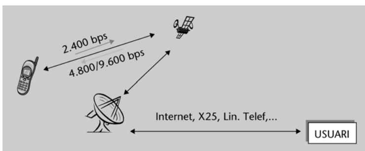
Orbcomm
