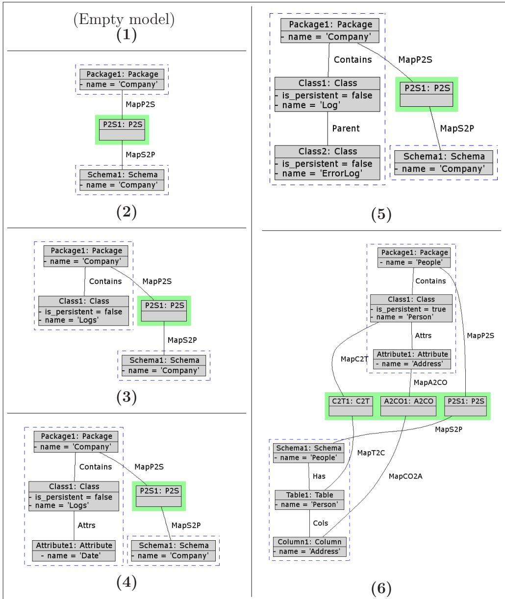
Figure 11: Sample TGG validation scenarios generated automatically, where the following rules are not source-enabled: Package- Schema (scenario 1), Class-Table (scenarios 1-5), ChClass-Table (scenarios 1-6) and Attribute-Column (scenarios 1-5).
