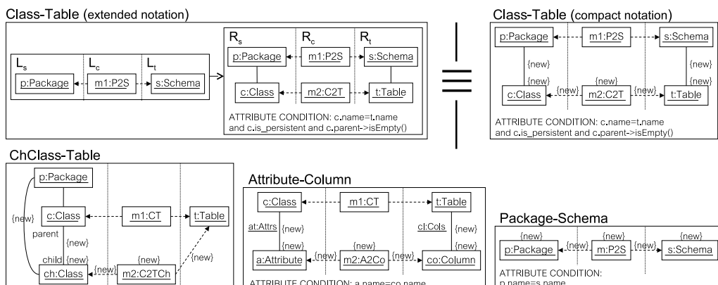
Figure 3: Some declarative TGG rules for the class-to-relational transformation.
