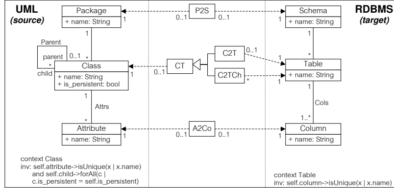
Figure 2: Example meta-model triple.
