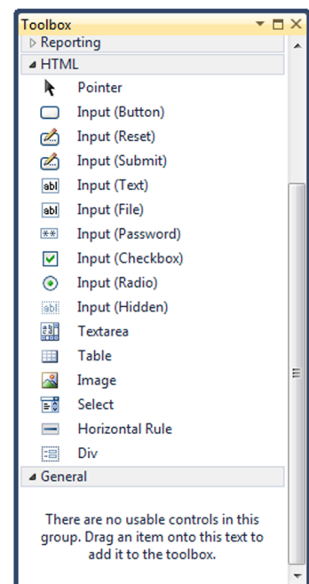
Figura 61. Controls HTML
