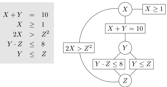
(a) Constraint system (b) Constraint network
