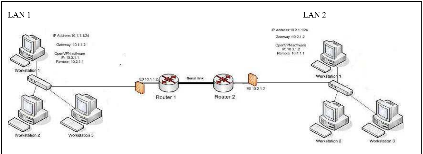
Figure 2: The WAN Test Network Design
