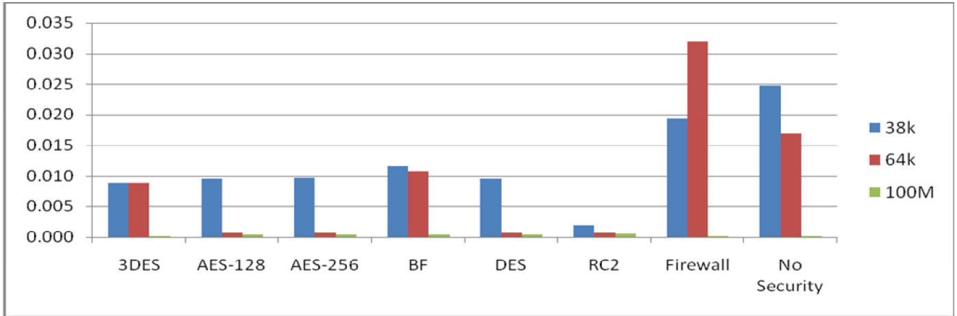
Figure 4: Degree of Jitter
