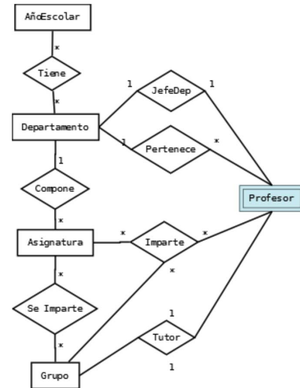
Diagrama E-R
