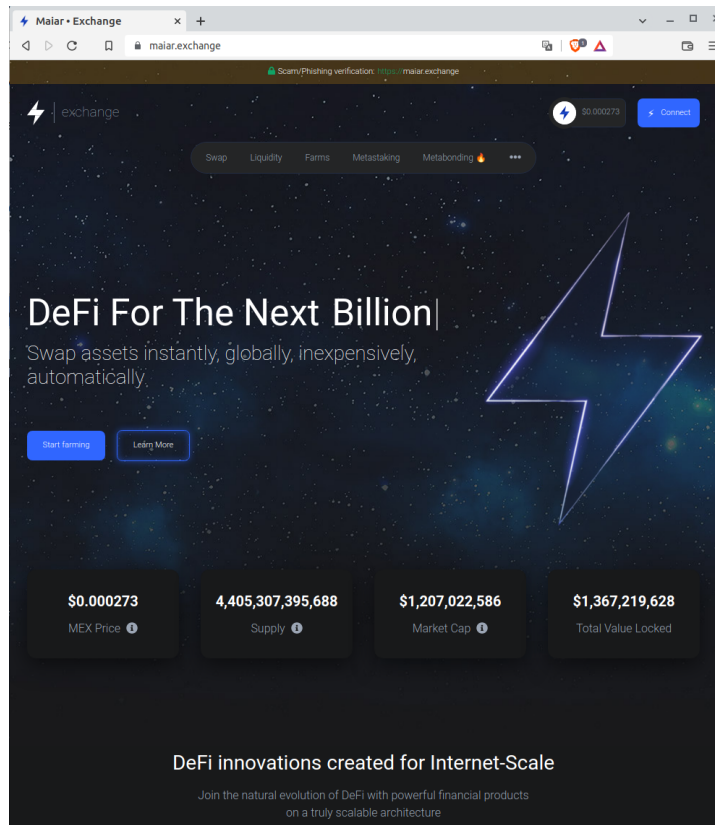
Figura 12: Maiar Exchange.
