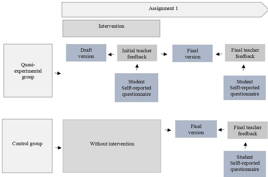
Fig. 1 Quasi-experiment procedure
