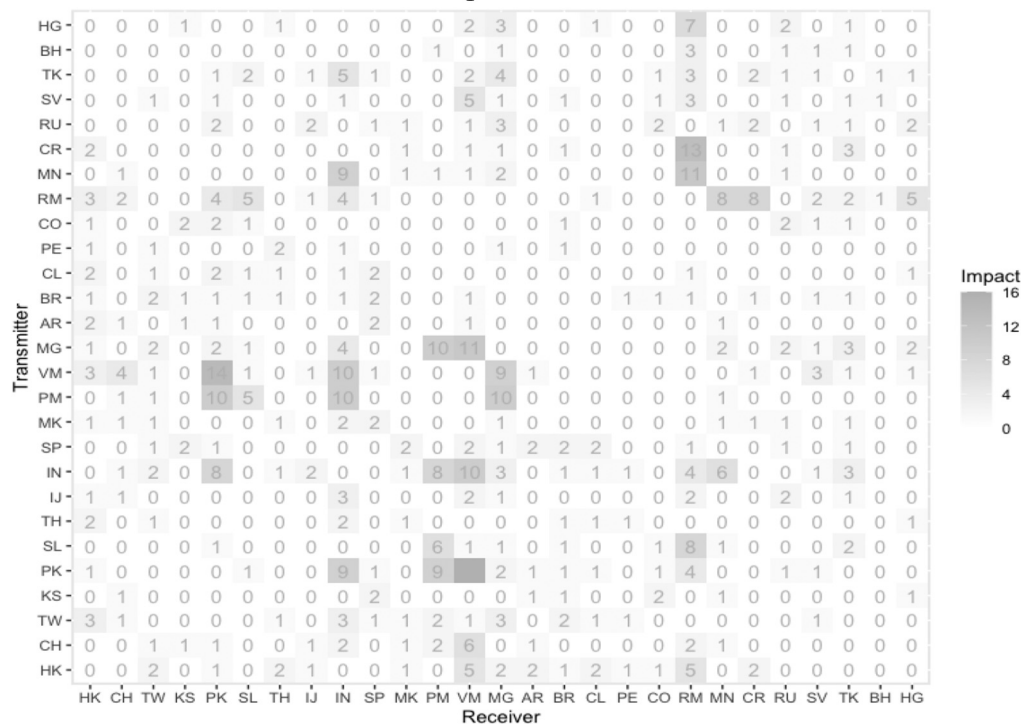
(b) Residual stock returns (after PCA)
