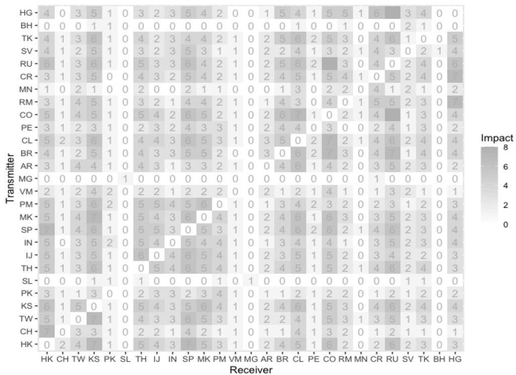
(b) Residual stock returns (after PCA)
