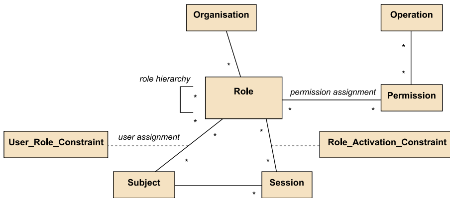
Figura 4. Model RBAC
