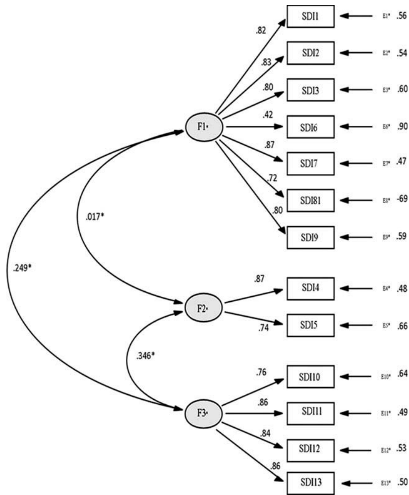
Figure 1. Path diagram of the three-factor model of the SDI.
