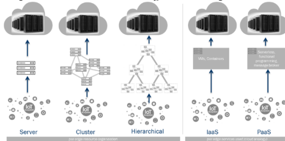
Fig. 8. Classification of Edge Computing models.
