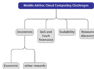
Fig. 5. Mobile Ad-hoc Cloud Computing Taxonomy.
