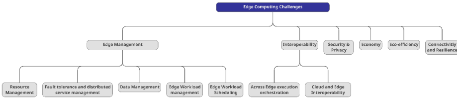
Fig. 7. Edge Computing Taxonomy.
