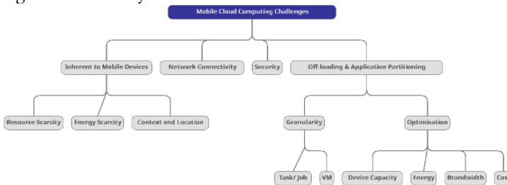
Fig. 3. Mobile Cloud Computing Taxonomy.
