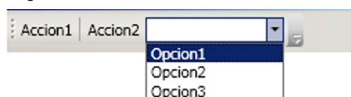
Figura 23. Control ToolBar
